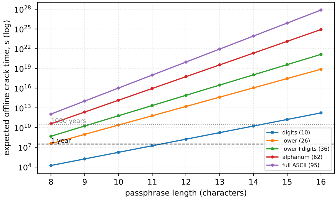
Crack time vs length at the fastest measured rate (2,927 cand/s, dual
