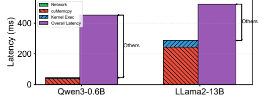
Figure 6: Performance Breakdown
