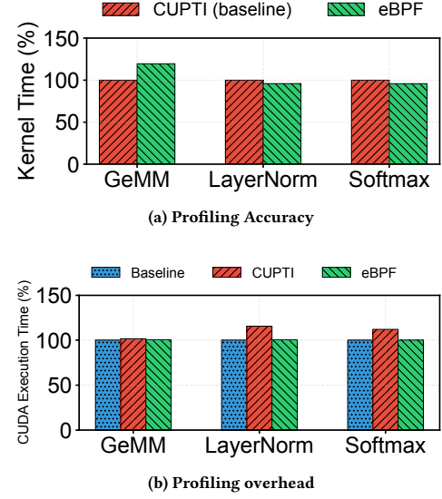
Figure 2: Profiling Results
