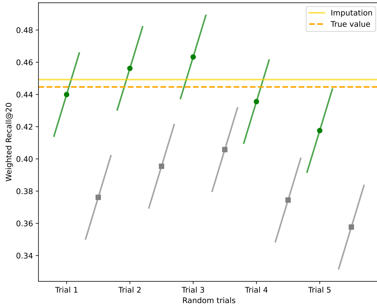
Confidence intervals (n=1000)
