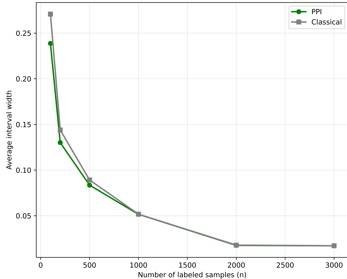
Interval width vs sample size
