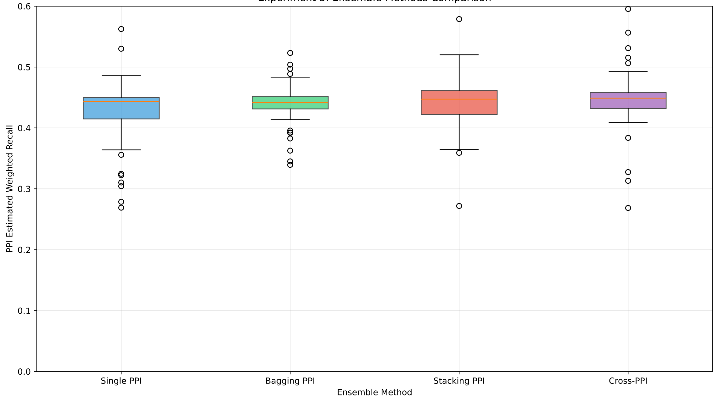
Experiment 5: Ensemble Methods Comparison
