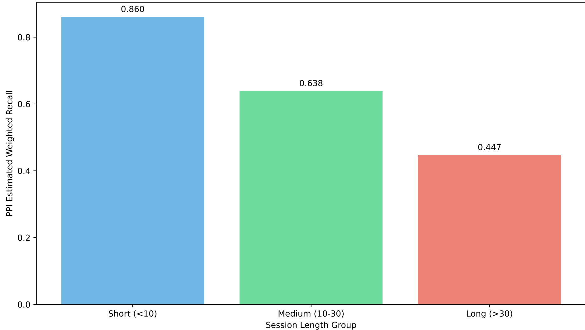
PPI Evaluation Results by Session Length
