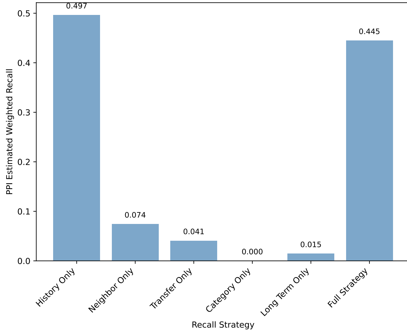
PPI Evaluation Results by Strategy
