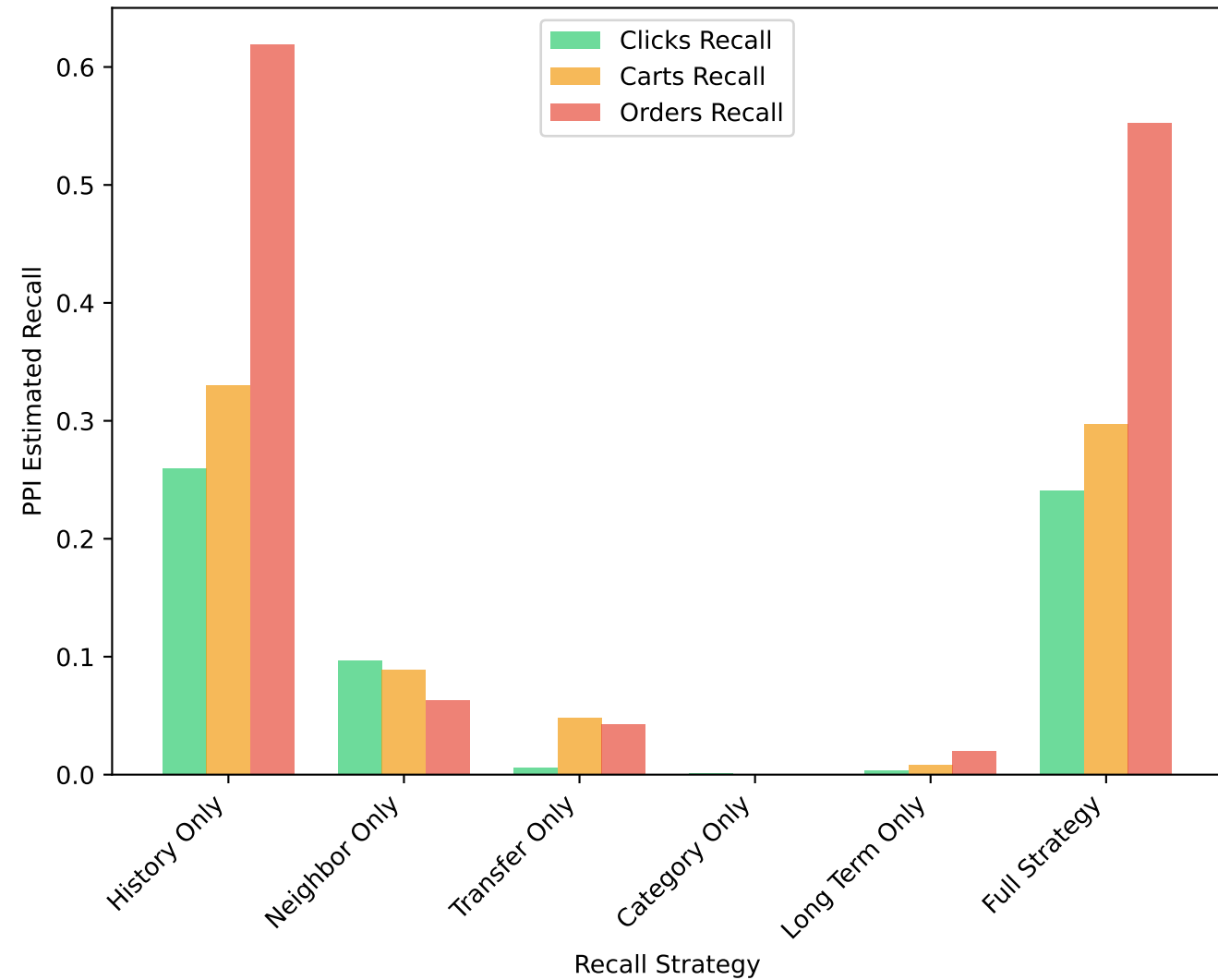
Recall by Strategy and Action Type
