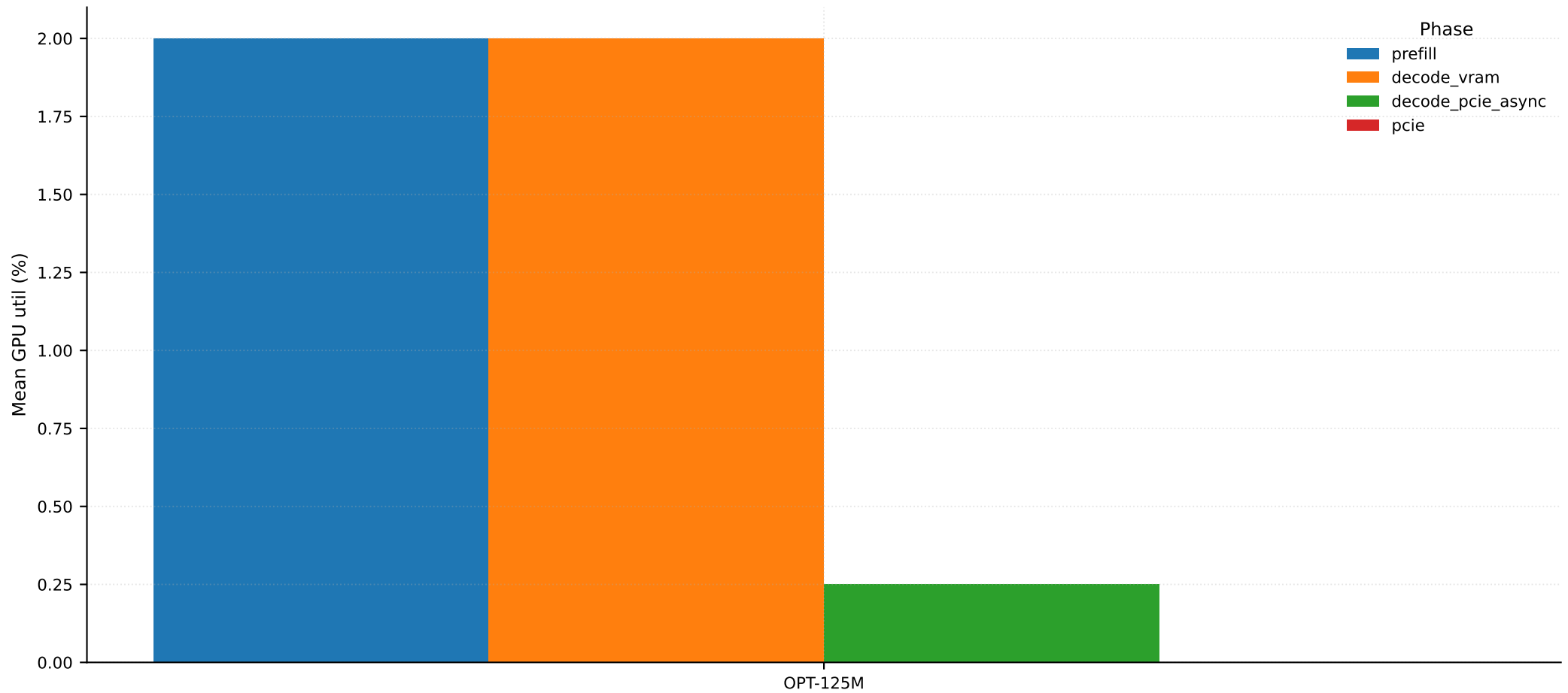
Revised hardware utilization profiling (mean GPU utilization by phase)
