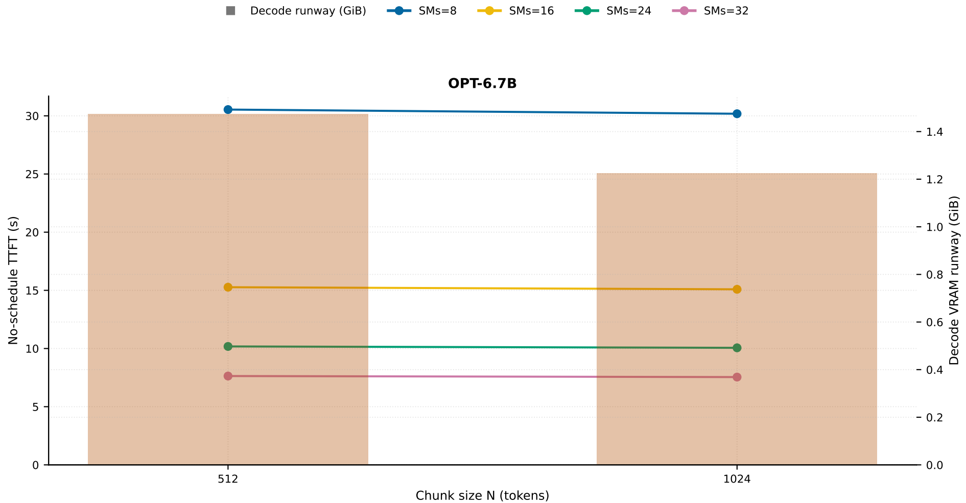
TTFT vs. runway trade-off (no schedule, by SM_AI)
