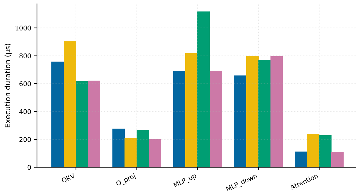
Decode · Duration
