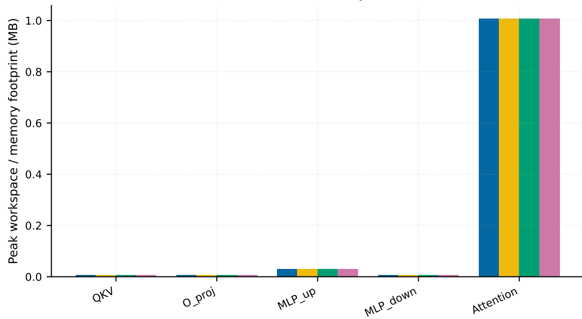
Decode · Workspace
