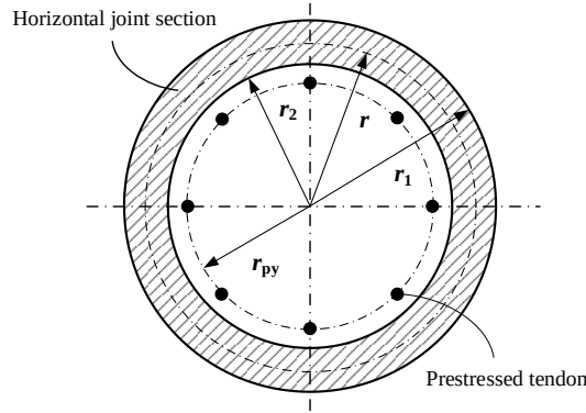
Fig 10 Horizontal joint cross-sectional geometric properties.
