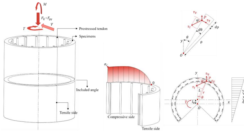
Fig. 21 Calculation diagram for the torsional capacity of horizontal joints
