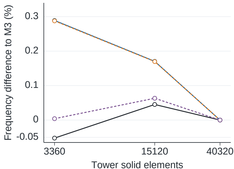
(c) Mesh volume effect
