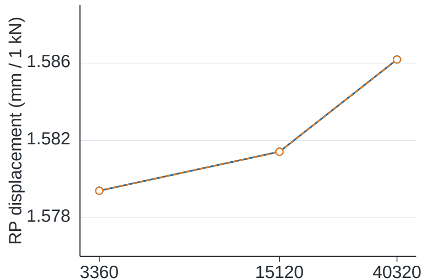
(b) Tangent flexibility
