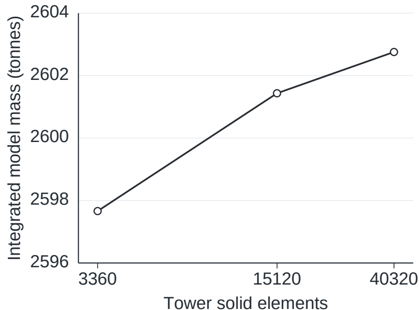
(c) Mesh volume effect
