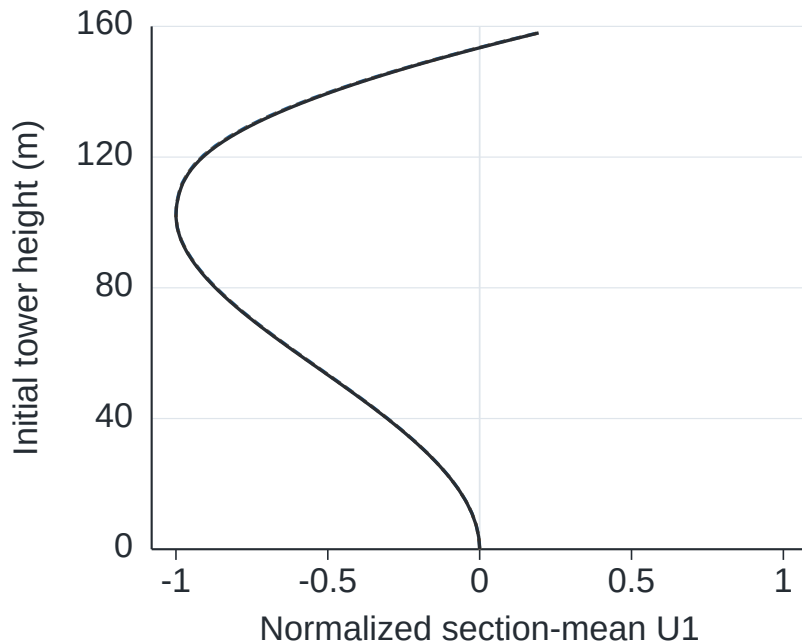
(c) Mode 3: X; M3 f = 0.70763 Hz
