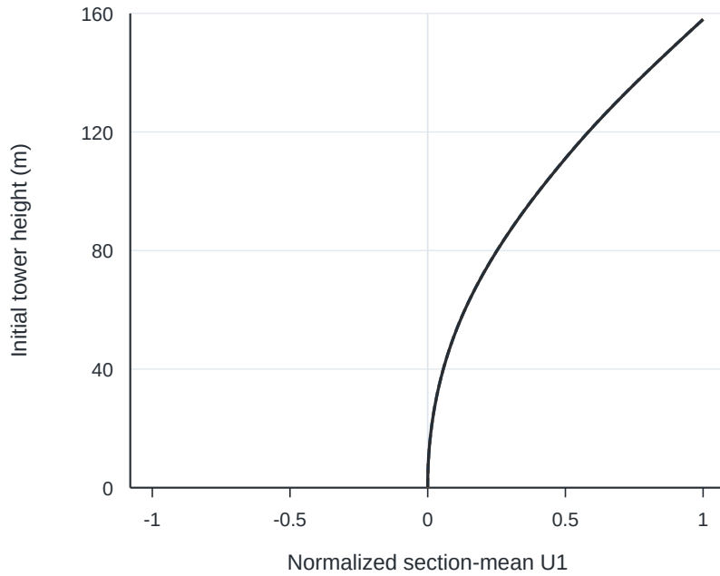
(c) Mode 3: X; M3 f = 0.70763 Hz
