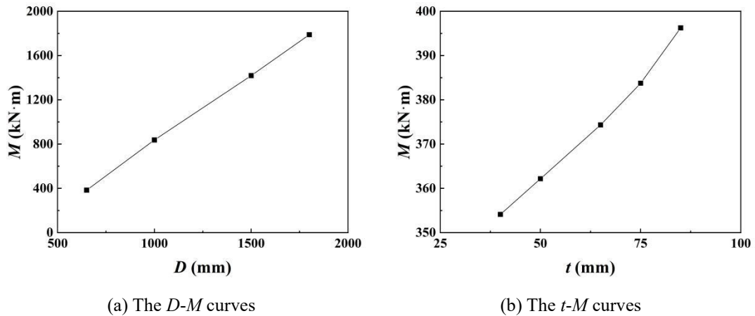
(a) The D - M curves (b) The t - M curves Fig 7 Effects of the geometric dimensions for compression-bending capacity.
