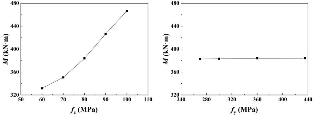
(a) The f_c - M curves (b) The f_y - M curves Fig 6 Effects of the material strength for compression-bending capacity.
