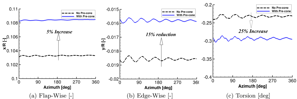
Figure 15: Azimuthal variations of the normalized blade-tip deformations
