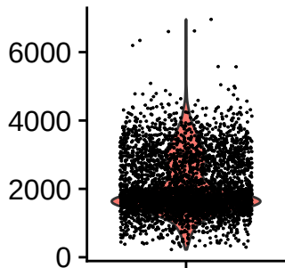
nFeature_RNA
