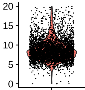
percent.mt
