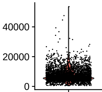
nCount_RNA
