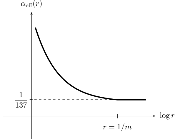
Figure 5.2: A qualitative sketch of the effective electromagnetic coupling constant generated by the one-loop vacuum polarization diagram, as a function of distance. The horizontal scale covers many orders of magnitude. Reference: Peskin [4] page 257.
