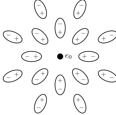
Figure 5.1: Virtual e^+e^- pairs are effective dipoles of length \sim 1/m , which screen the bare charge of electron. The reference is Peskin and Schroeder [4] at page 255 figure 7.8.
