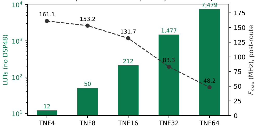
TNF multiplier on XC7A200T, one cycle of latency
