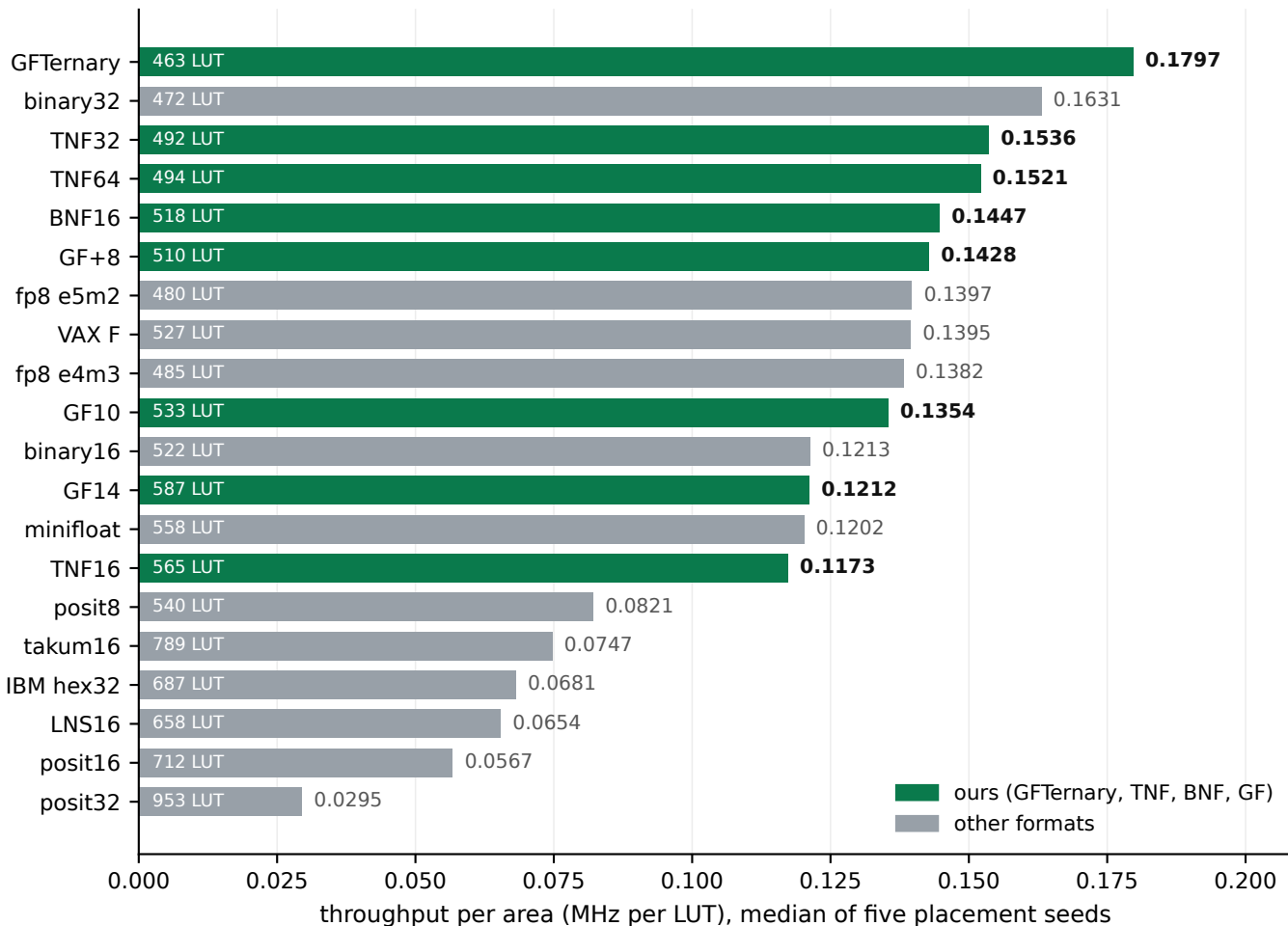
One ternary-neuron datapath, XC7A200T, no DSP, whole accumulator observed
