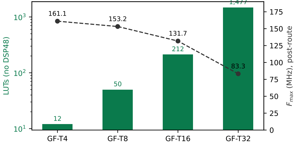
GF-T multiplier on XC7A200T, one cycle of latency
