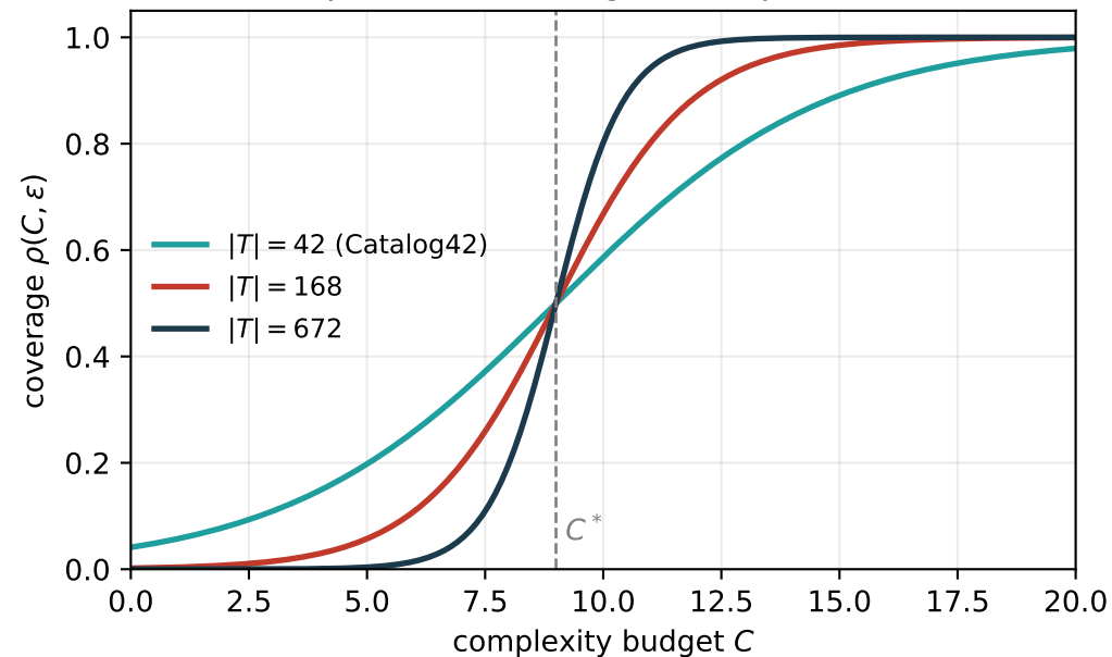
Conjectured coverage order parameter
