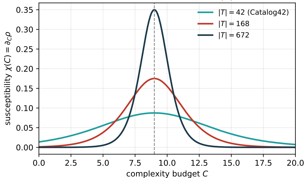
Susceptibility peak; width \sim |T|^{-1/2}
