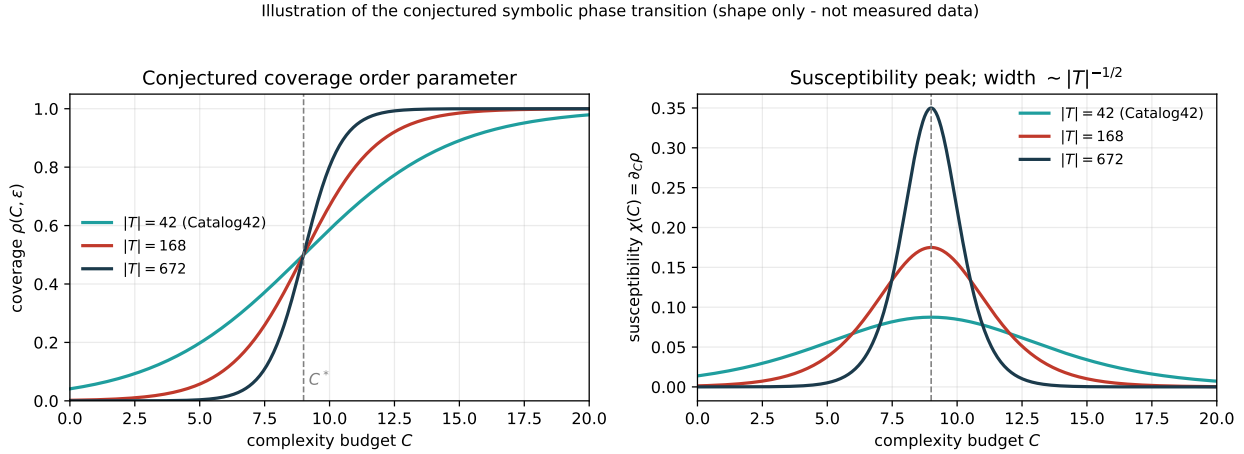
Figure 1: Illustration of the conjectured symbolic phase transition (Section 4.4). Left: the coverage order parameter \rho(C, \epsilon) sharpens as the target-set size |T| grows. Right: the susceptibility \chi(C) = \partial_C \rho develops a taller, narrower peak at C^* , with width scaling as |T|^{-1/2} . These are the conjectured shapes, not measured data; the figure exists to make the falsifiable prediction visual.
