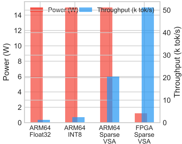
(a) Power vs Throughput
