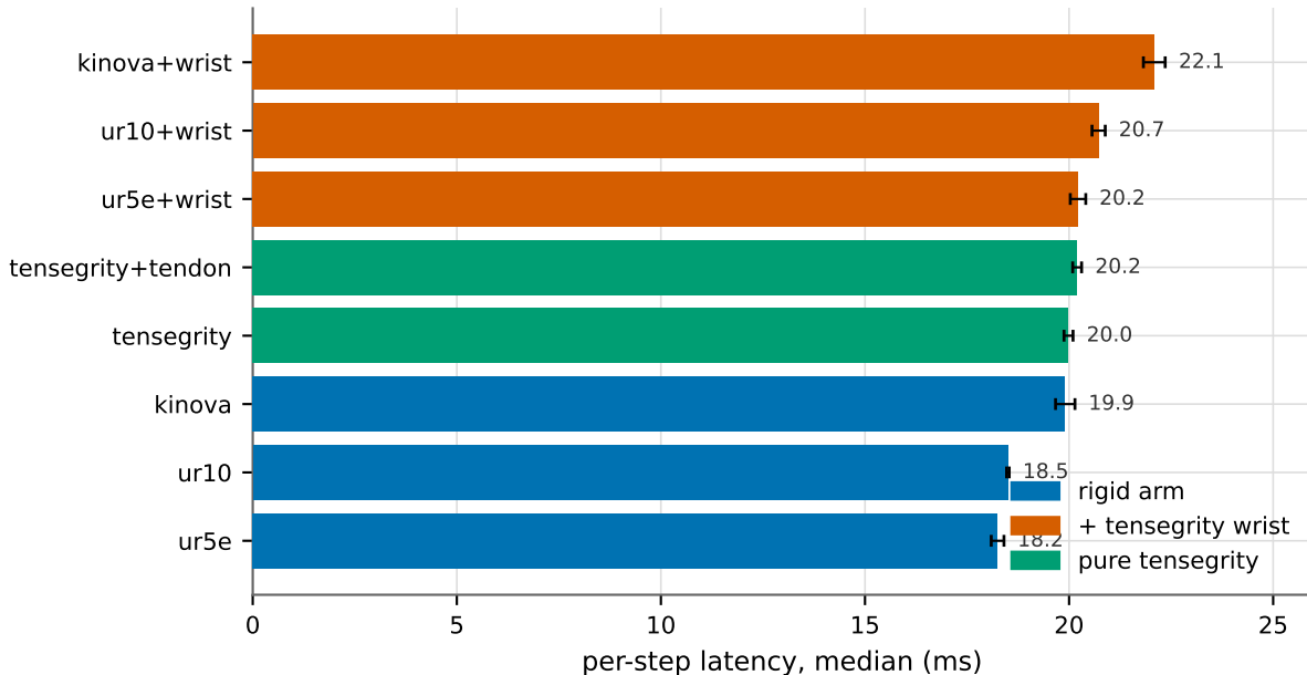
Robot morphology / DOF cost (reach, N=1024)
