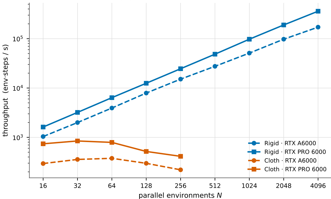
Cross-GPU throughput: RTX A6000 vs. RTX PRO 6000 (Blackwell)
