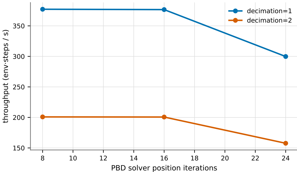
Optimisation lever: solver iterations × decimation
