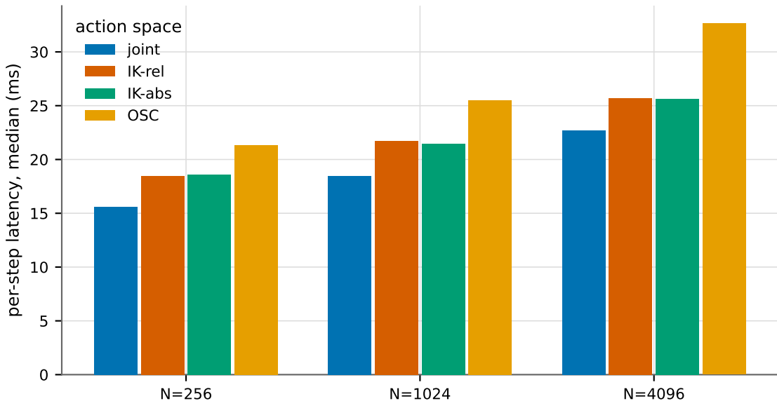
Action-space controller cost (UR5e reach)
