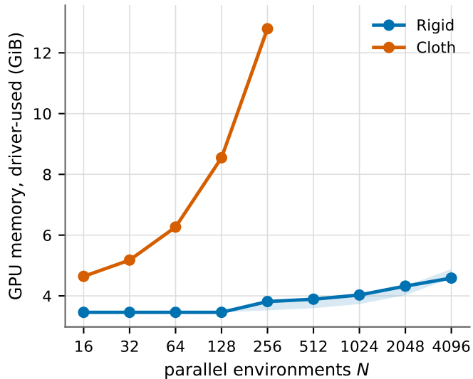
GPU memory footprint
