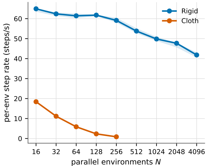
Per-environment step rate
