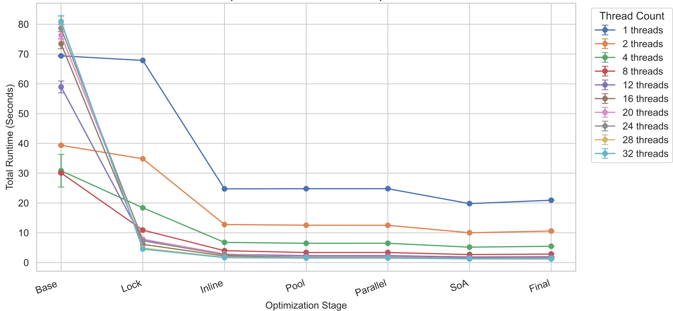
Total Time Performance Progression — Scene: 02-Cornell-Box (95% Confidence Intervals)
