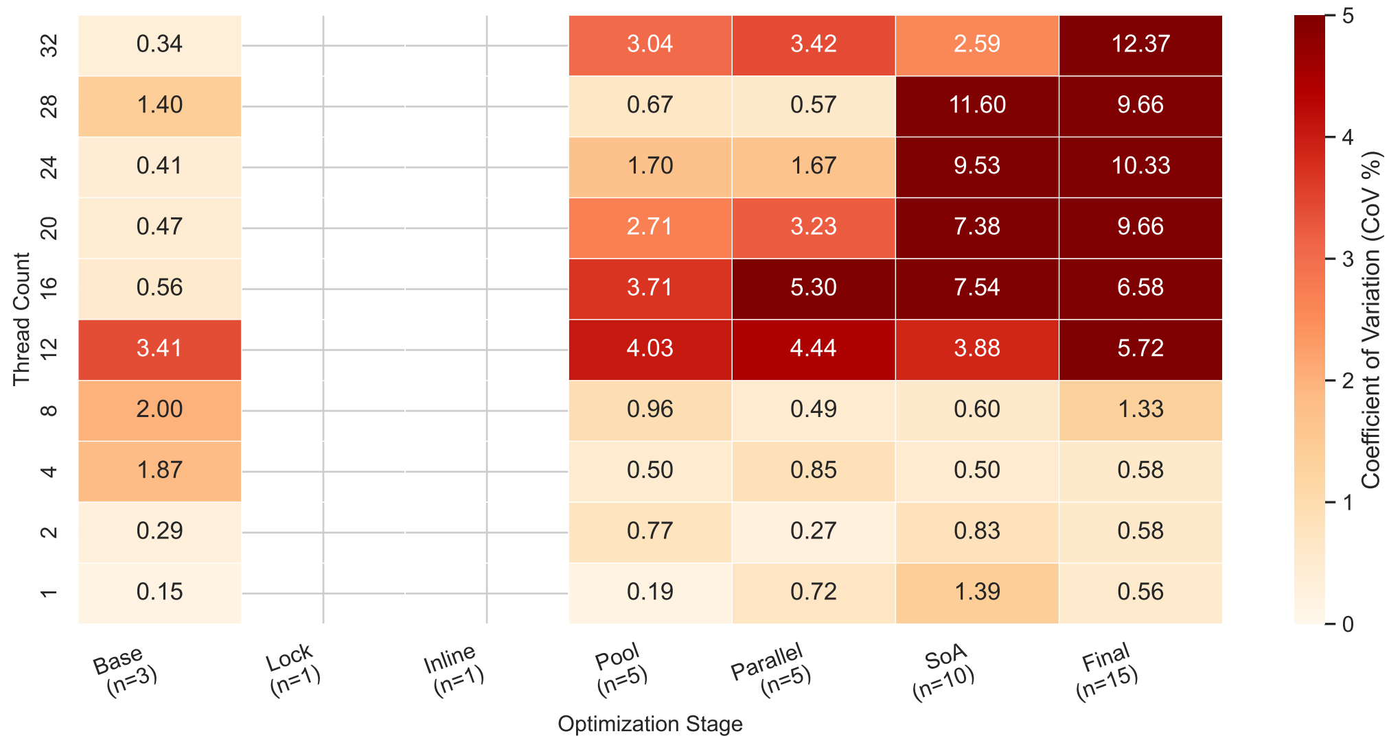
Benchmark Run Stability Heatmap (CoV%) — Scene: 01-Box (CoV Range: 0% - 5%)
