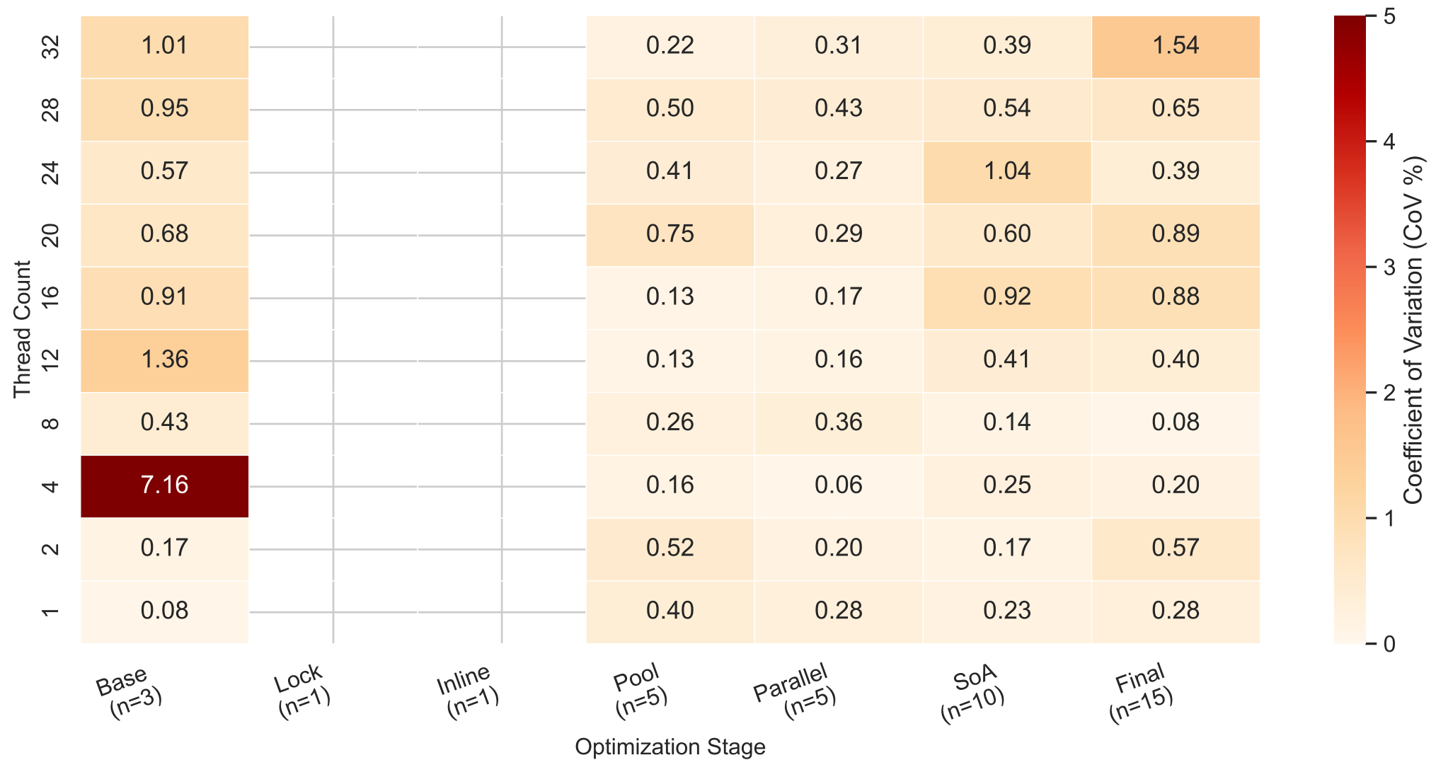
Benchmark Run Stability Heatmap (CoV%) — Scene: 02-Cornell-Box (CoV Range: 0% - 5%)
