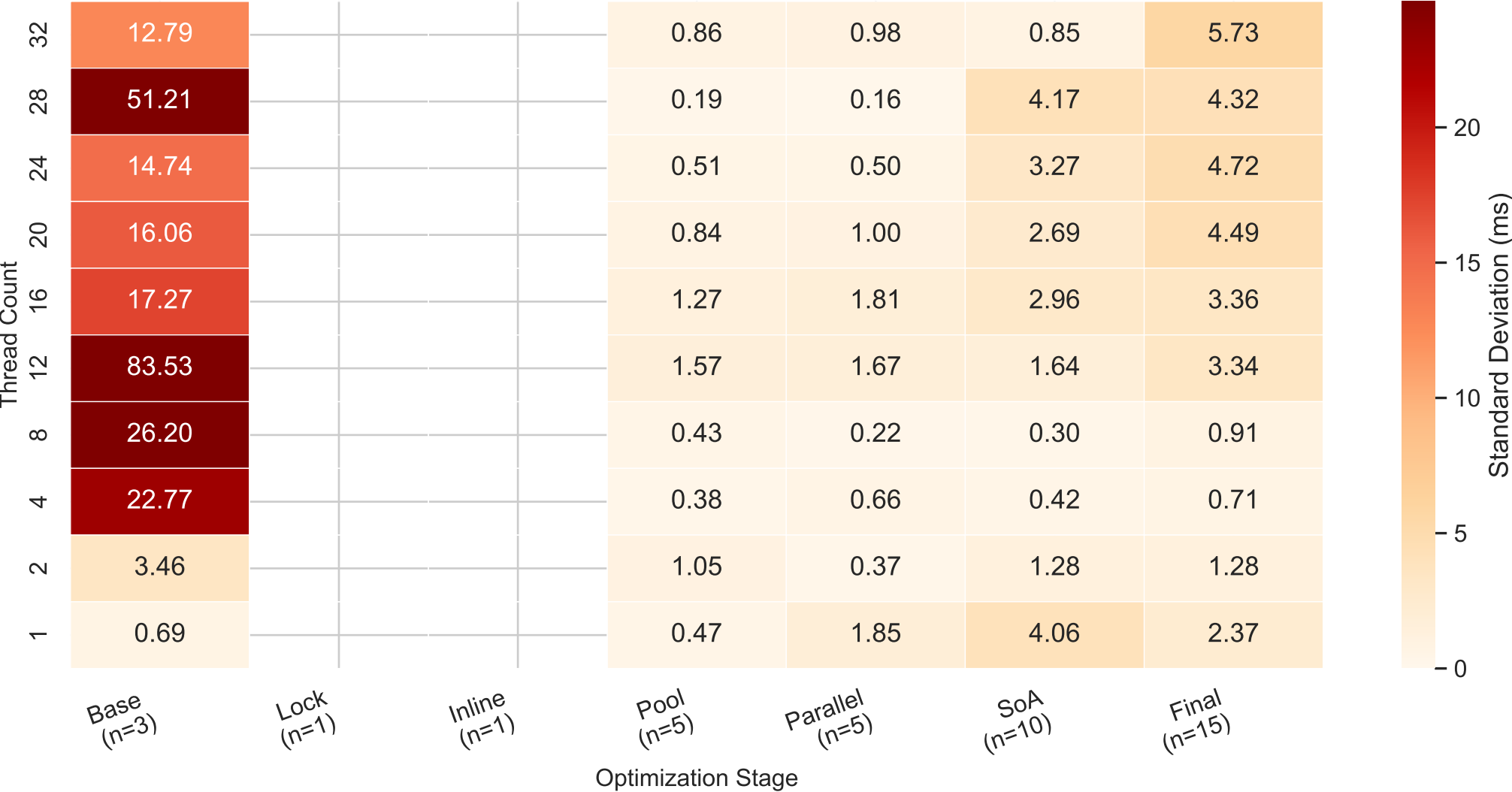
Benchmark Run Stability Heatmap (Std Dev) — Scene: 01-Box (Std Dev Range: 0 – 24.65 ms)
