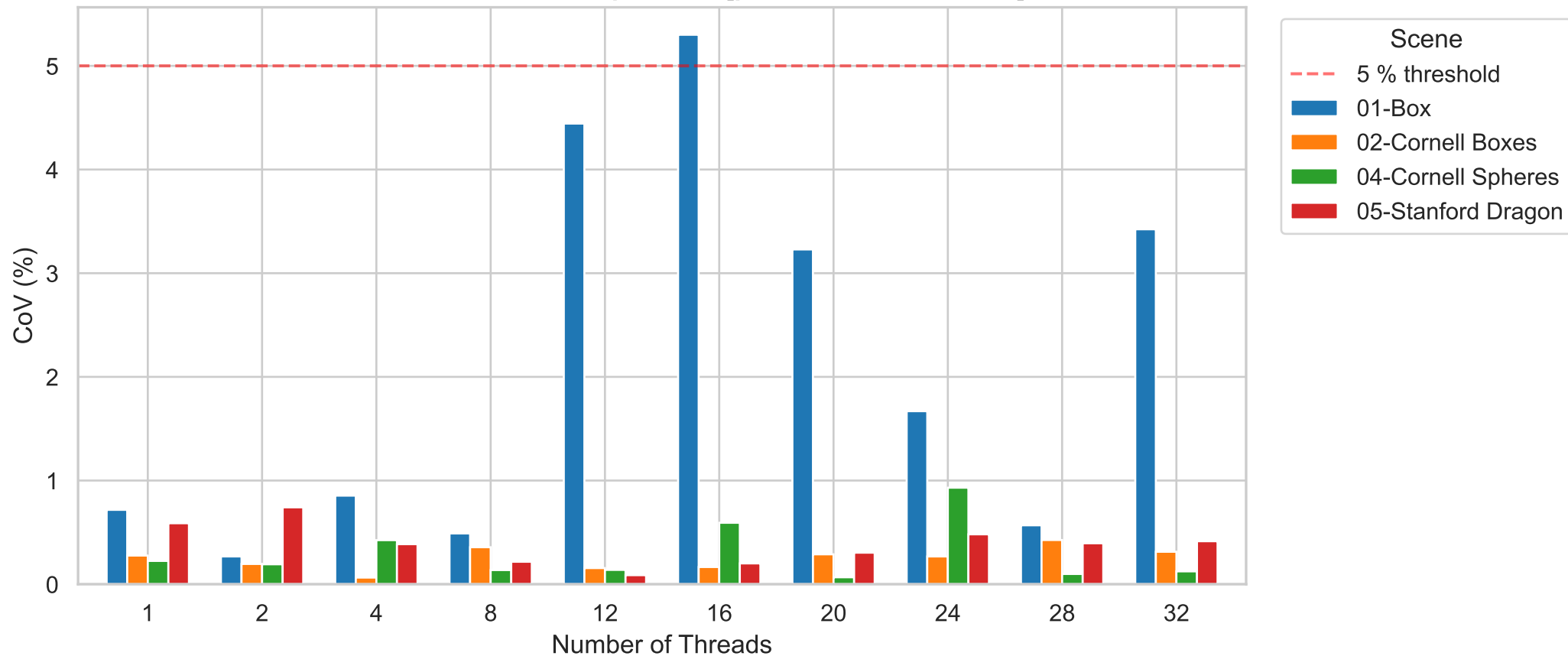
Total Time CoV across Repetitions [parallel branch - 5 runs]
