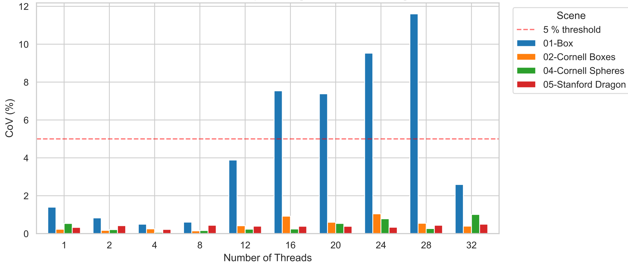
Total Time CoV across Repetitions [soa branch - 10 runs]
