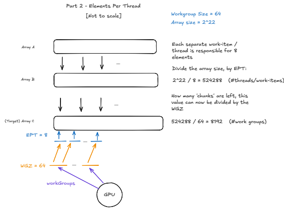
Figure 6: Elements per thread (8) - Work Item Orchestration
