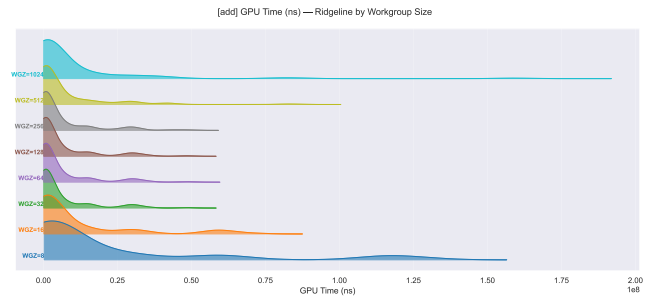
Figure 16: Ridgeline Visualization of the GPU time in function of workgroup-size
