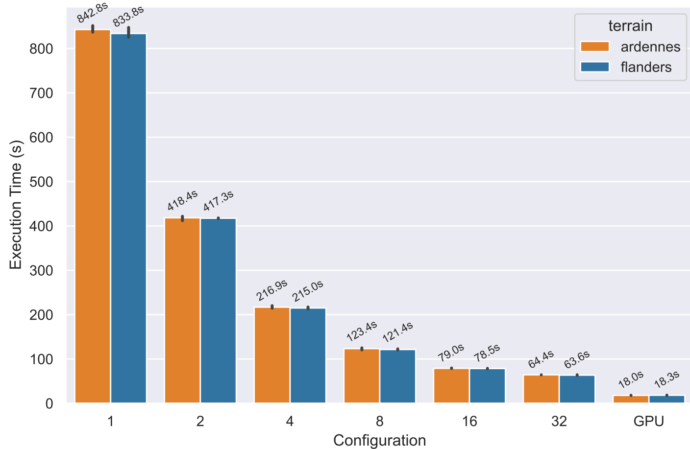
Execution Time Population=1000 | Generations=100 | Sensors=100
