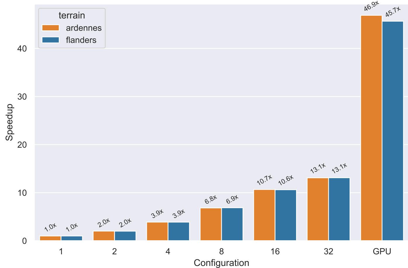
Speedup Population=1000 | Generations=100 | Sensors=100
