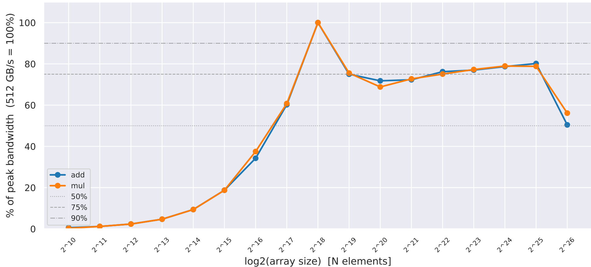
% of Peak Bandwidth Achieved vs Array Size
