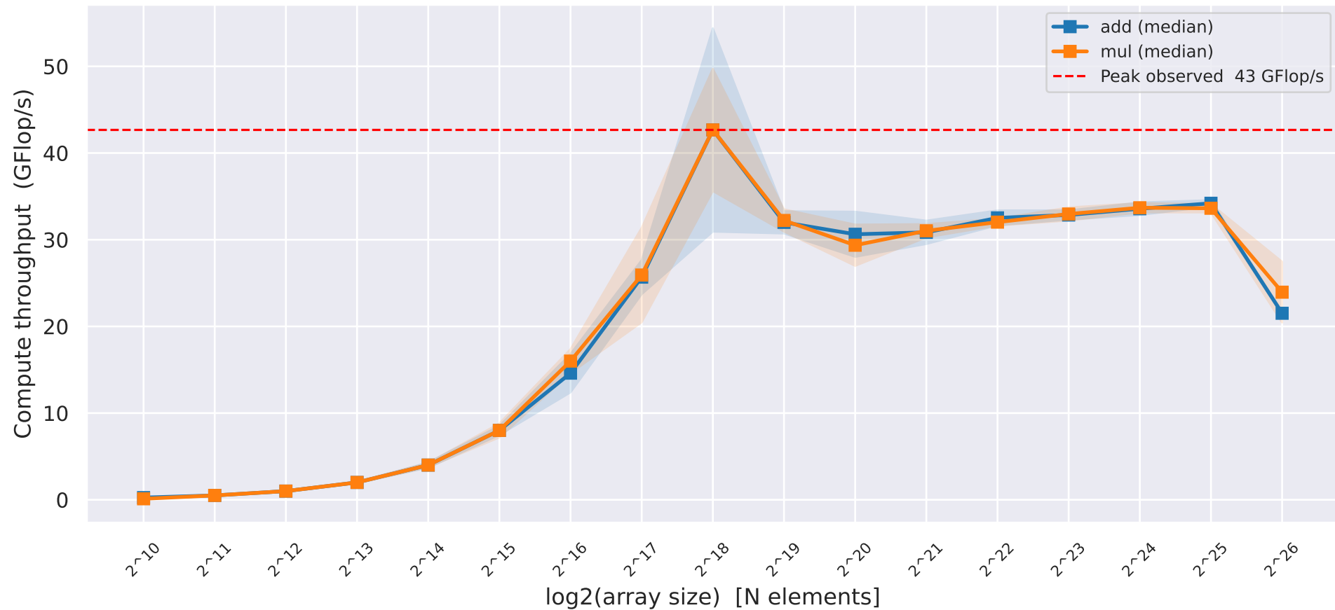
GPU Compute Throughput vs Array Size
