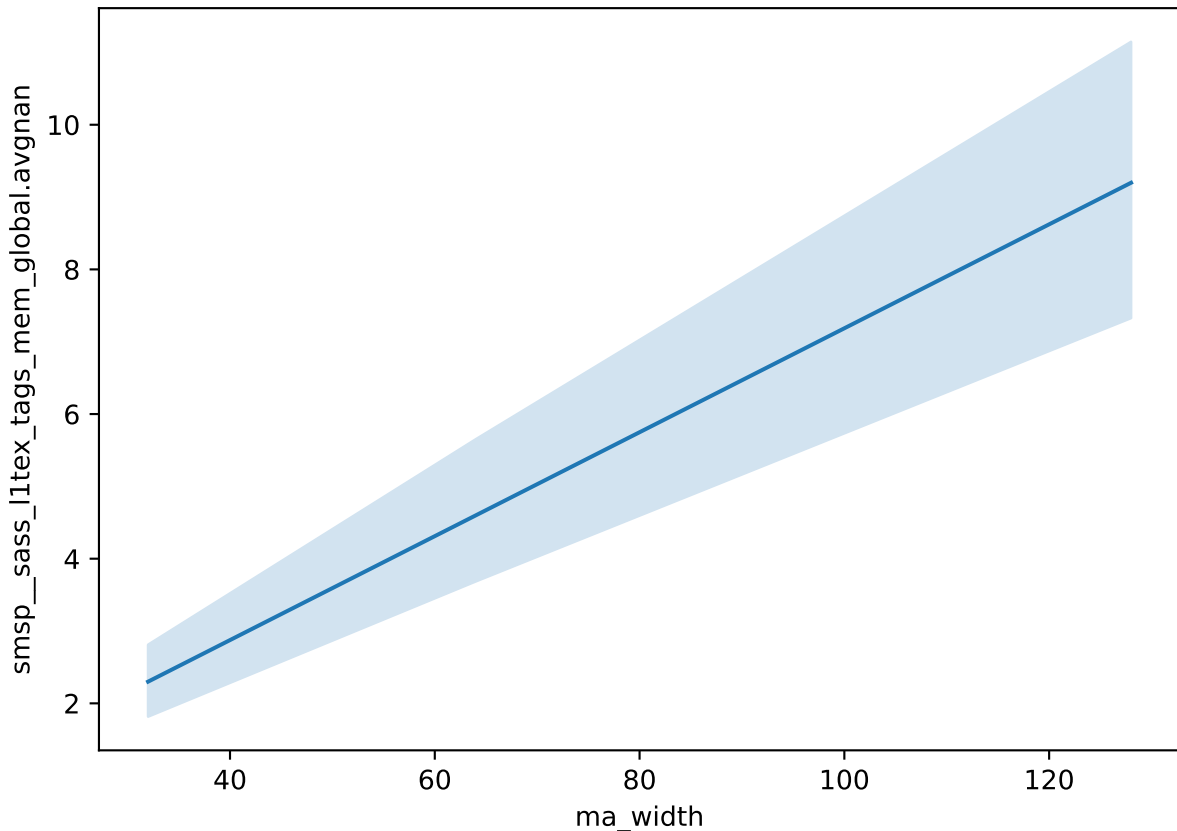
Matrix A Size vs NCU Metrix
