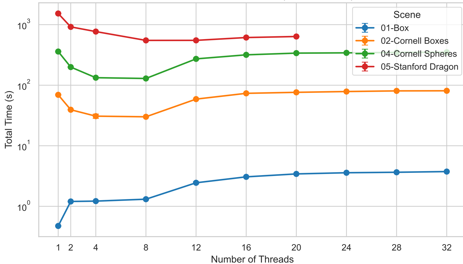
Total Time vs Thread Count (mean \pm 2·SEM)
