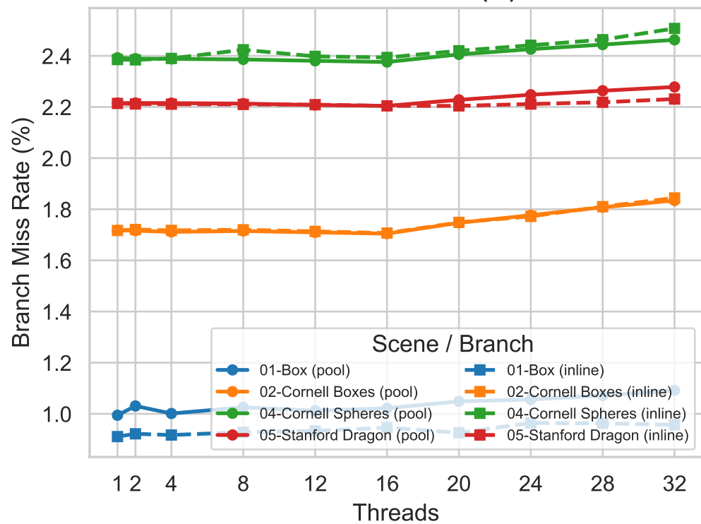
Branch Miss Rate (%)
