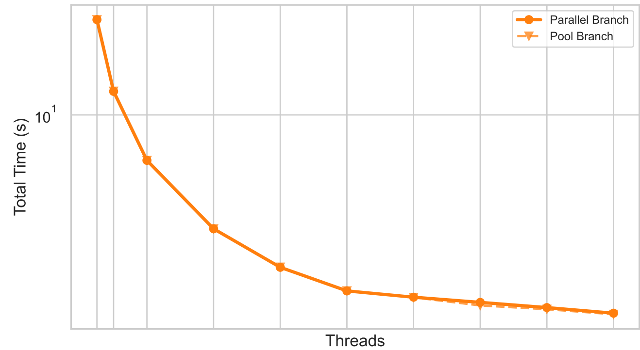
05-Stanford Dragon
