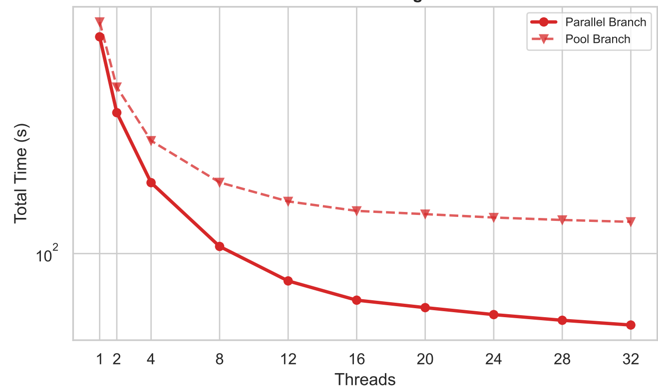
05-Stanford Dragon
