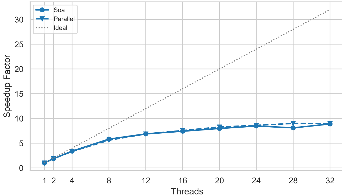
04-Cornell Spheres
