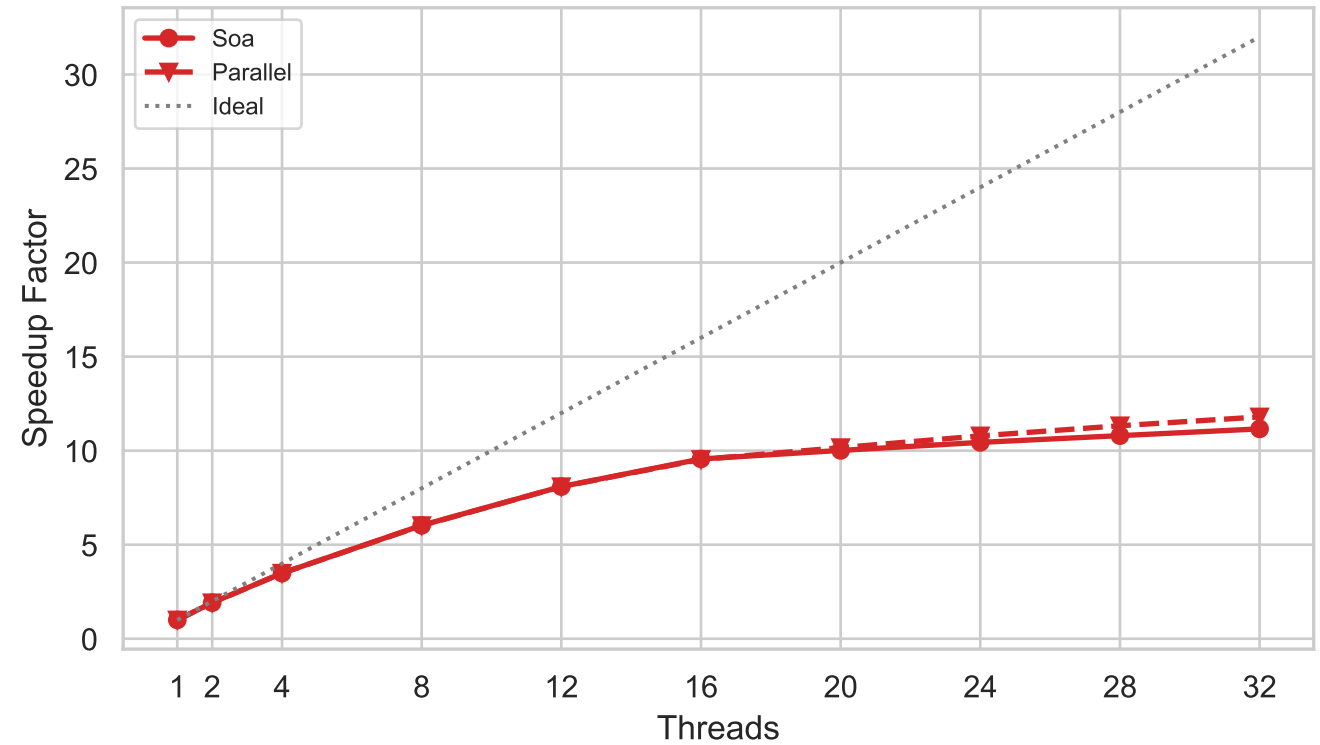
05-Stanford Dragon
