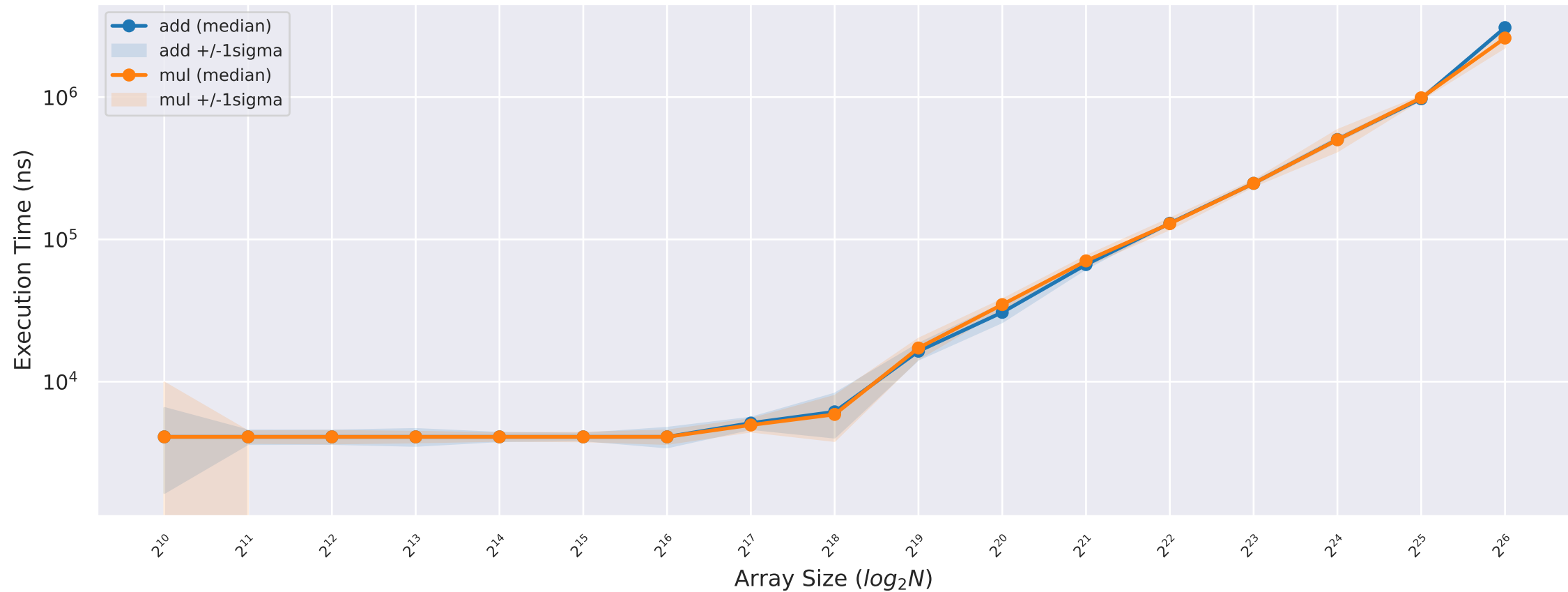
GPU Execution Time vs Array Size
