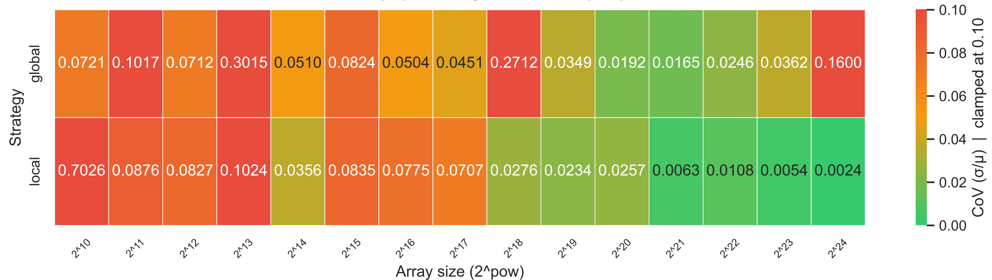
GPU Time (ns) CoV — global vs local [add]
