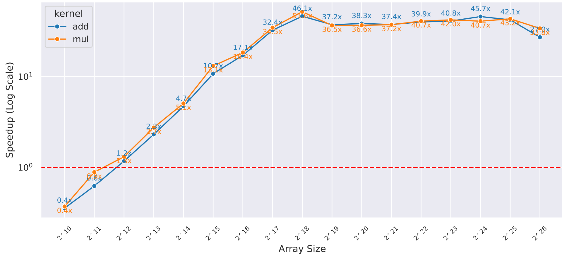
GPU Speedup Factor over CPU
