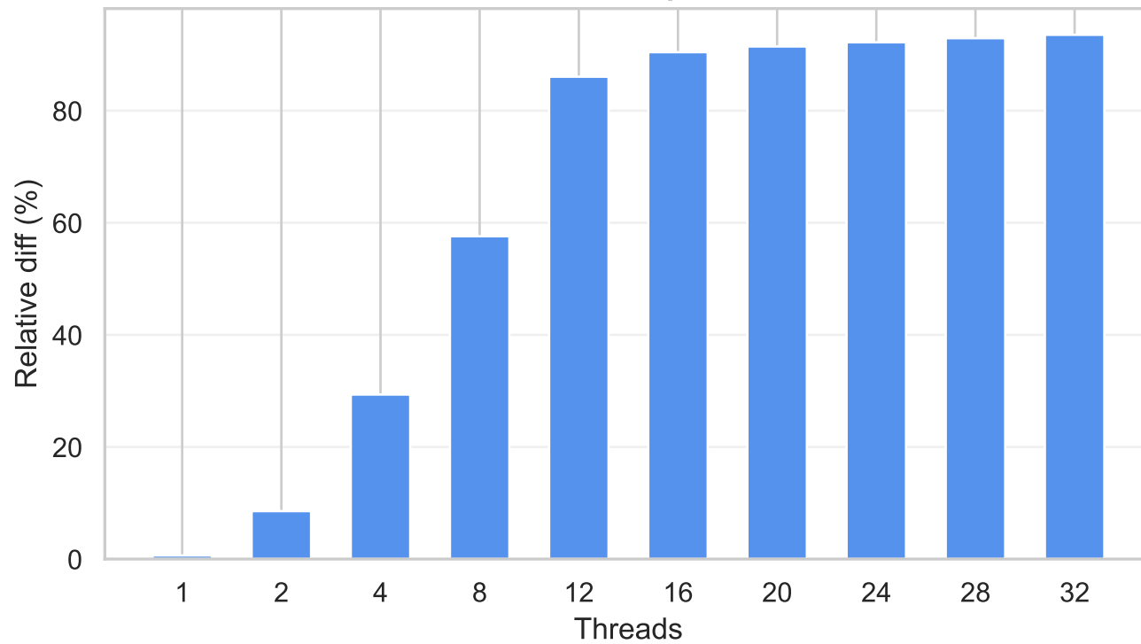
04-Cornell Spheres
