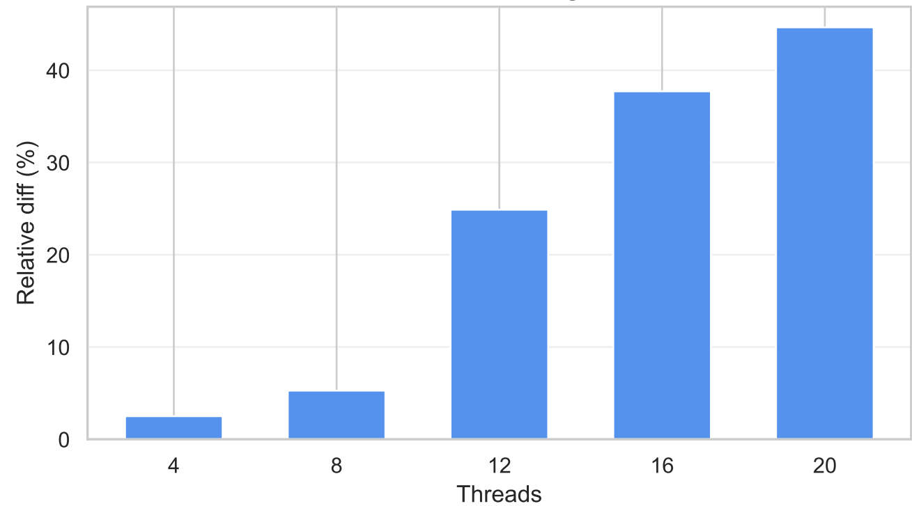
05-Stanford Dragon
