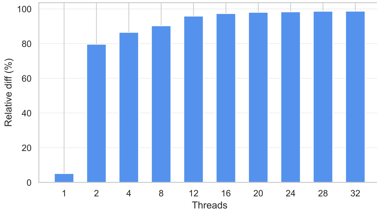
04-Cornell Spheres
