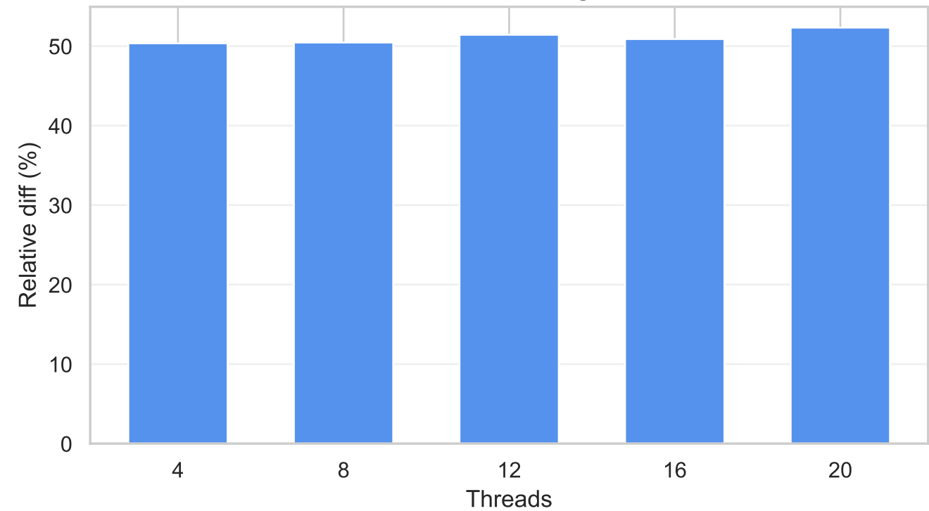
05-Stanford Dragon
