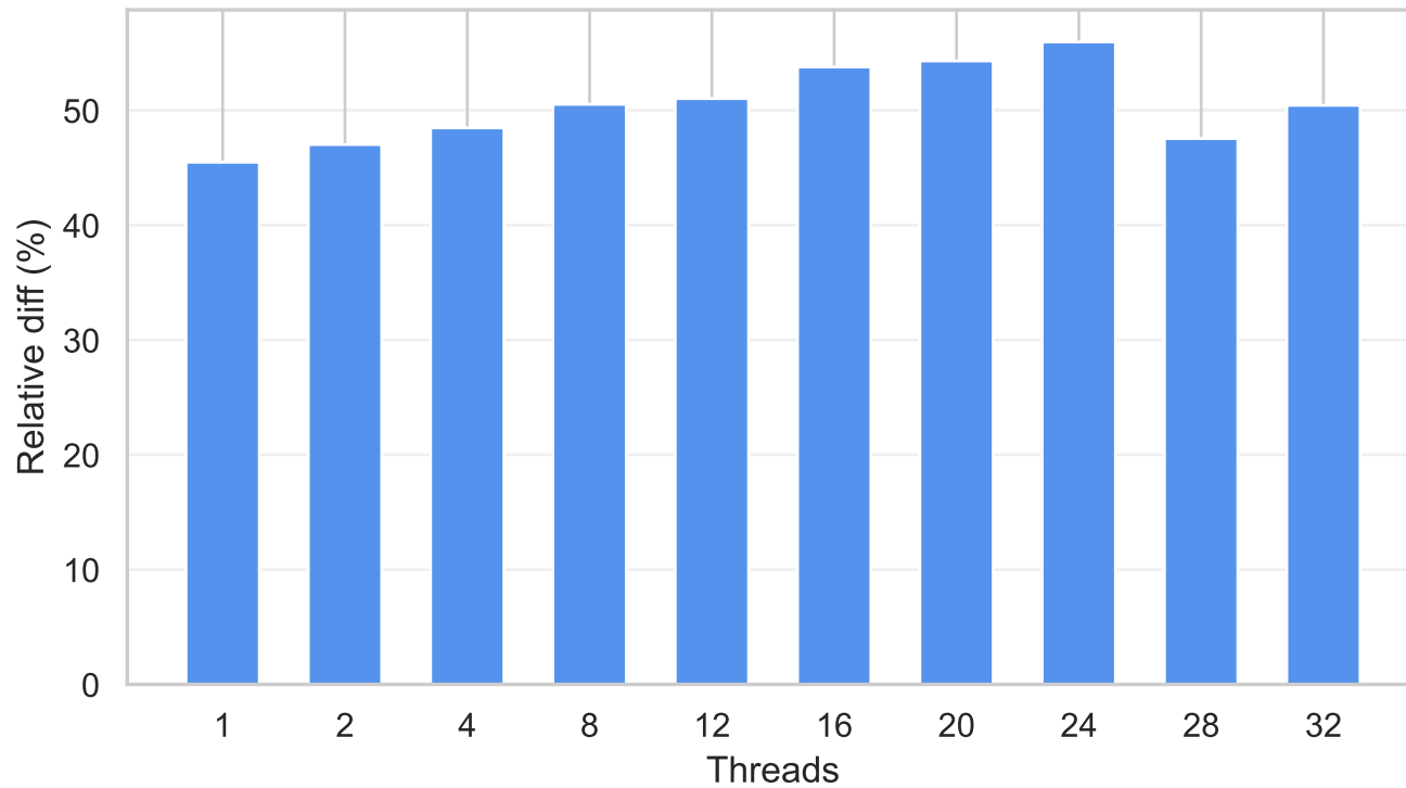
04-Cornell Spheres
